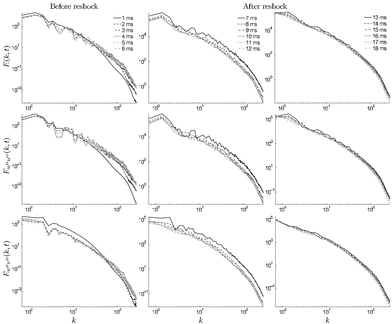
FIG. 12. The time evolution of the total, streamwise, and spanwise fluctuating kinetic energy spectra E(k, t) (top row), E_{u''u''}(k, t) (middle row), and E_{v''v''}(k, t) (bottom row), respectively, at 1 ms intervals (in units of \text{cm}^3/\text{s}^2 ). The spectra before reshock are shown in the first column and the spectra after reshock are shown in the second and third columns.
