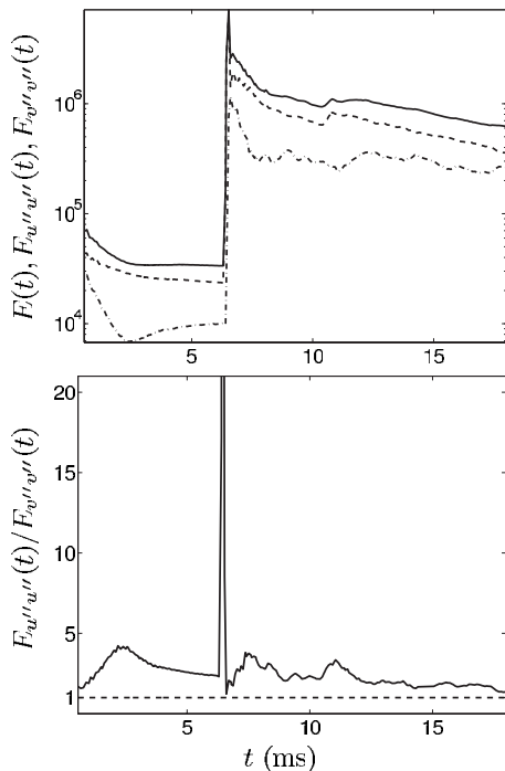
FIG. 19. The time evolution of the fluctuating kinetic energy E(t) (solid line) and its streamwise and spanwise components E_{u'u'}(t) and E_{v'v'}(t) (dashed and dot-dashed lines, respectively) (in units of \text{cm}^2/\text{s}^2 ) (top), and the time evolution of the ratio of the streamwise and spanwise component of the fluctuating kinetic energy E_{u'u'}(t)/E_{v'v'}(t) (bottom).
