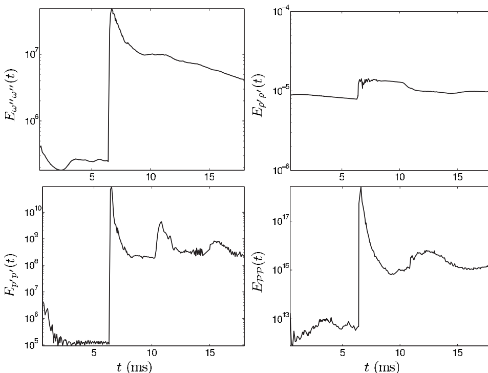
FIG. 20. The time evolution of the fluctuating enstrophy E_{\omega'\omega'}(t) (in units of \text{s}^{-2} ), density variance E_{\rho'\rho'}(t) (in units of \text{g}^2/\text{cm}^6 ), pressure variance E_{p'p'}(t) (in units of \text{bar}^2 ), and baroclinic vorticity production variance E_{PP}(t) (in units of \text{s}^{-4} ).
