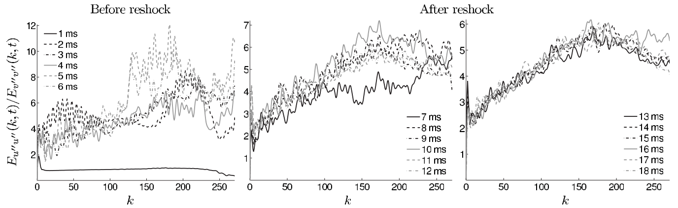
FIG. 13. The time evolution of the ratio of the streamwise and spanwise fluctuating kinetic energy spectra E_{u'u''}(k, t)/E_{v''v''}(k, t) before and after reshock at 1 ms intervals. The ratios before reshock are shown in the first column and the ratios after reshock are shown in the second and third columns.
