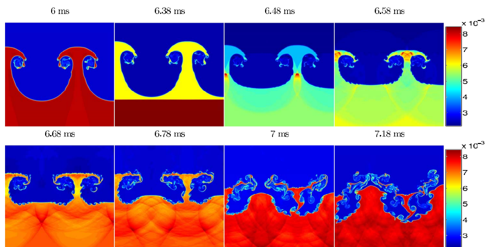
FIG. 1. (Color online) The density fields (in units of \text{g/cm}^3 ) at 6, 6.38, 6.48, 6.58, 6.58, 6.68, 6.78, 7, and 7.18 ms. The gases are air (acetone) (top) and \text{SF}_6 (bottom).
